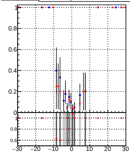
— DQM_mkFit_time — DQM_BDT_mkFit_time
