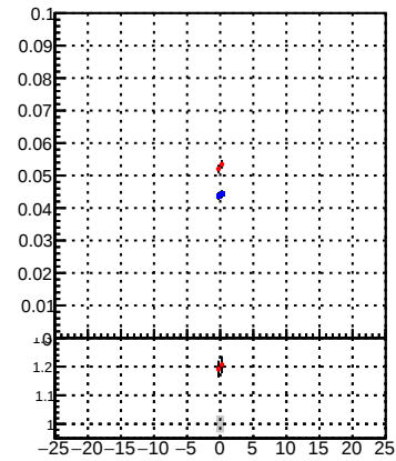
—●— DQM_mkFit_time —●— DQM_BDT_mkFit_time
