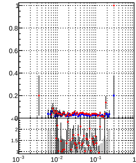
Fake rate vs \mu DQM_mkFit_time DQM_BDT_mkFit_time
