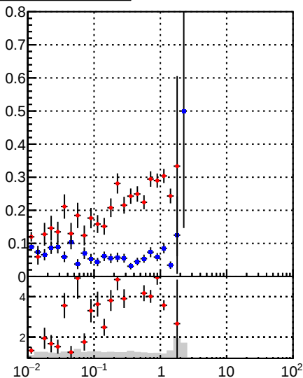
—•— DQM_mkFit_time —•— DQM_BDT_mkFit_time
