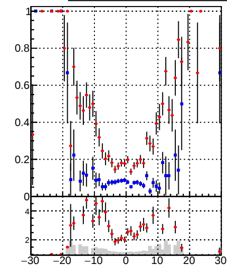
—●— DQM_mkFit_time —●— DQM_BDT_mkFit_time
