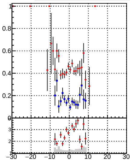
—•— DQM_mkFit_time —•— DQM_BDT_mkFit_time
