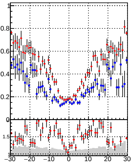
—●— DQM_mkFit_time —●— DQM_BDT_mkFit_time
