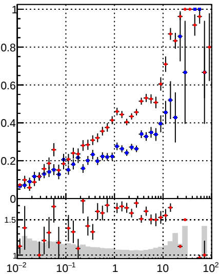
—●— DQM_mkFit_time —●— DQM_BDT_mkFit_time
