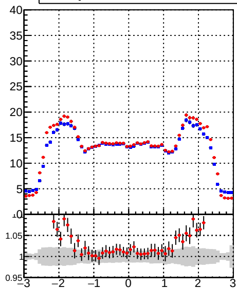
mean hit DQM_mkFit_time DQM_BDT_mkFit_time
