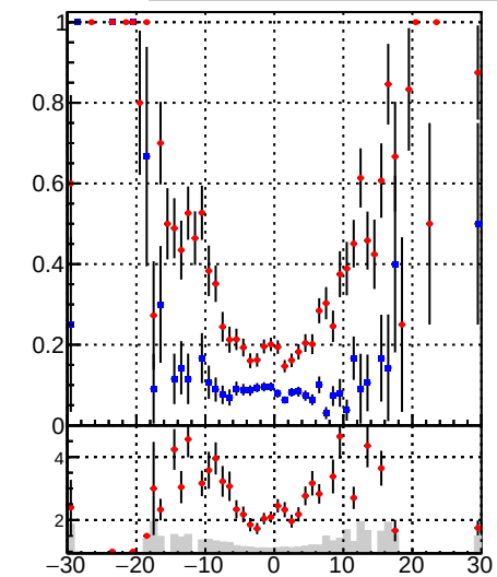
— DQM_mkFit_time — DQM_BDT_mkFit_time
