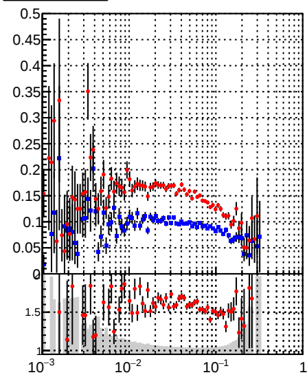
—•— DQM_mkFit_time —•— DQM_BDT_mkFit_time
