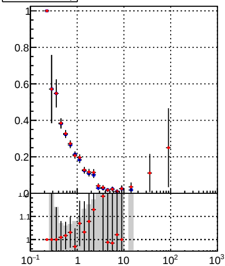
—•— DQM_mkFit_time —•— DQM_BDT_mkFit_time
