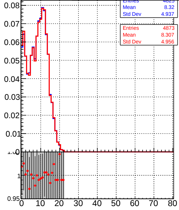
Legend: DQM_mkFit_time (grey shaded area), DQM_BDT_mkFit_time (red line with diamonds)
