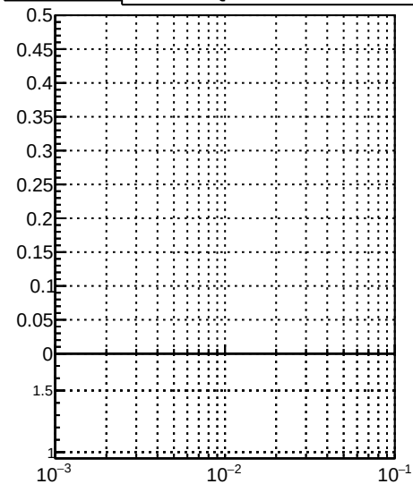
Fake rate vs \sqrt{s} DQM_mkFit_time DQM_BDT_mkFit_time
