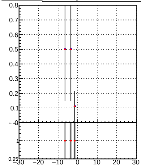
Fake rate vs v Legend: DQM_mkFit_time (blue line with error bars), DQM_BDT_mkFit_time (red line with error bars)
