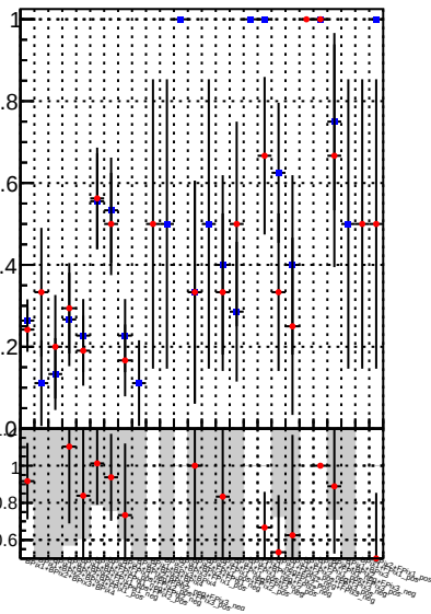
Fake rate vs. —●— DQM_mkFit_time —●— DQM_BDT_mkFit_time
