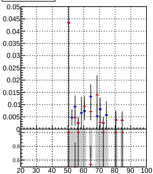
Efficiency vs pu
