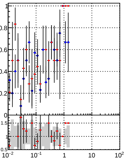
Fake rate vs v DQM_mkFit_time DQM_BDT_mkFit_time
