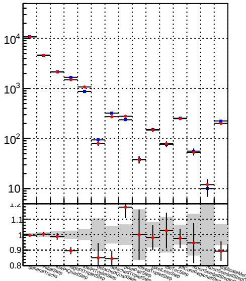
Number of Events Legend: DQM_mkFit_time DQM_BDT_mkFit_time
