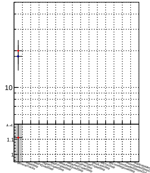
Number of Events Legend: DQM_mkFit_time DQM_BDT_mkFit_time
