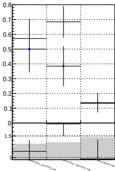
Fake rate vs. — DQM_mkFit_time — DQM_BDT_mkFit_time
