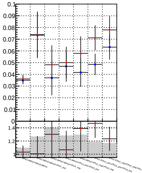
Fake rate vs. DQM_mkFit_time DQM_BDT_mkFit_time
