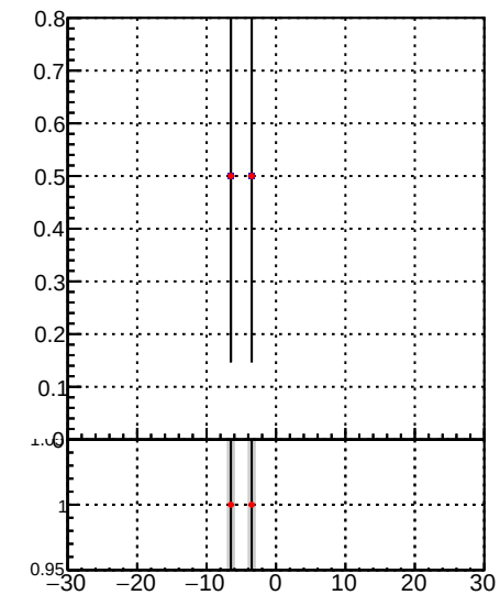
Fake rate vs d —•— DQM_mkFit_time —•— DQM_BDT_mkFit_time
