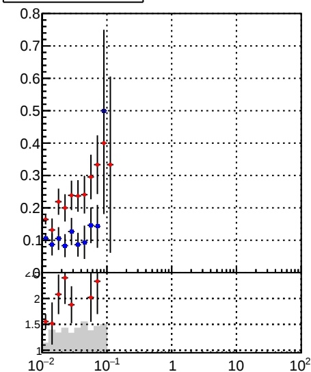
—•— DQM_mkFit_time —•— DQM_BDT_mkFit_time
