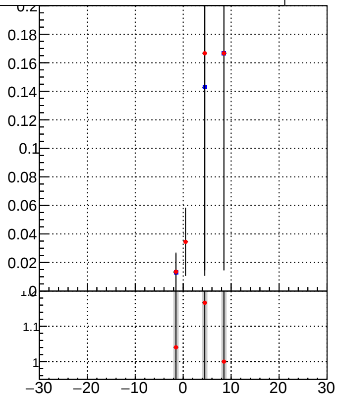
DQM_mkFit_time DQM_BDT_mkFit_time
