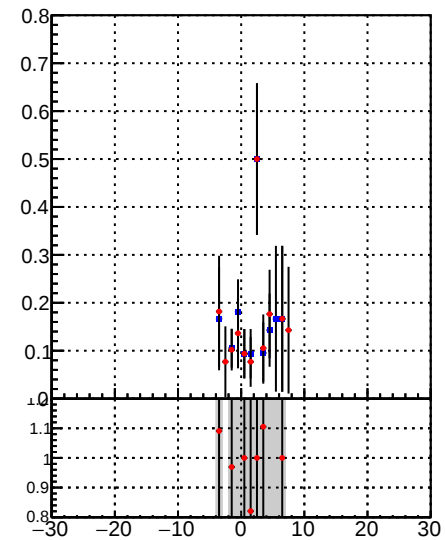
Fake rate vs d Legend: DQM_mkFit_time (blue dots) DQM_BDT_mkFit_time (red dots)
