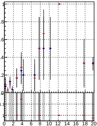
Fake rate vs. DQM_mkFit_time DQM_BDT_mkFit_time
