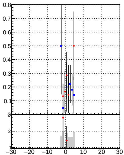
—●— DQM_mkFit_time —●— DQM_BDT_mkFit_time
