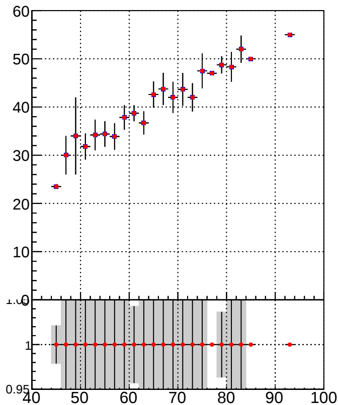
MatchedRecoVtx_vs_GenVtx
