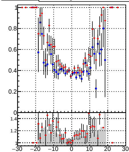
—●— DQM_mkFit_time —●— DQM_BDT_mkFit_time
