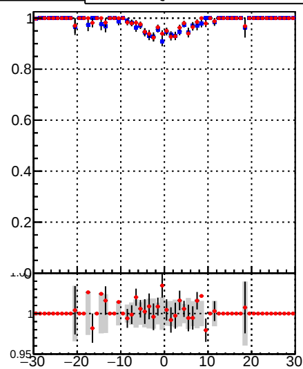
— DQM_mkFit_time — DQM_BDT_mkFit_time Fake rate vs v
