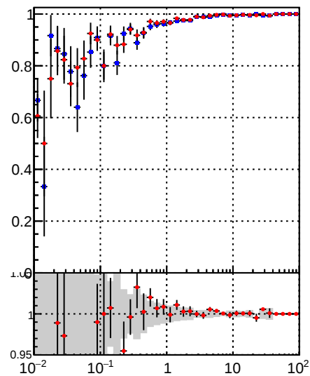
Fake rate vs v — DQM_mkFit_time — DQM_BDT_mkFit_time
