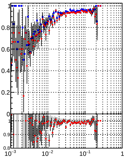
■ DQM_mkFit_time ● DQM_BDT_mkFit_time
