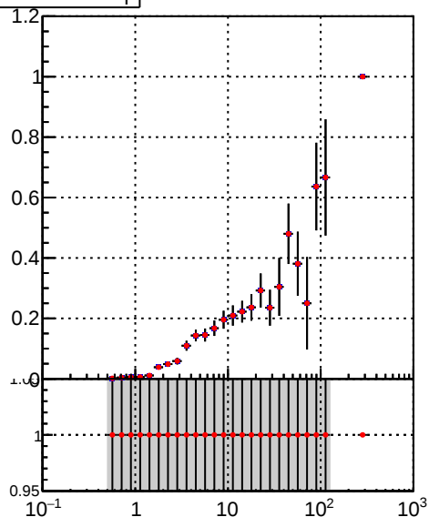
— DQM_mkFit_time — DQM_BDT_mkFit_time
