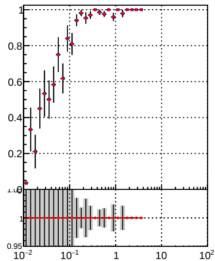
█ DQM_mkFit_time █ DQM_BDT_mkFit_time
