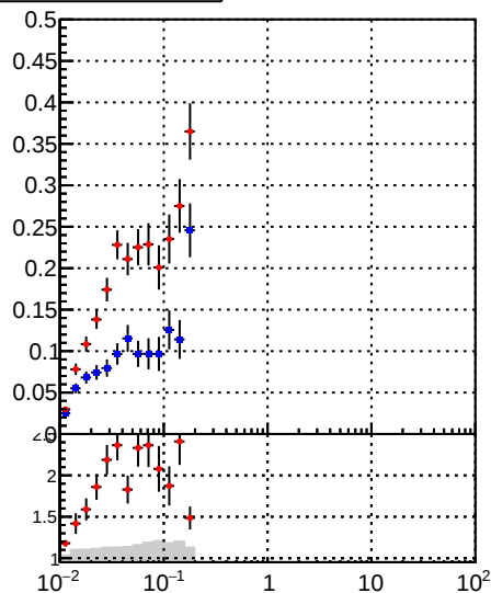
—●— DQM_mkFit_time —●— DQM_BDT_mkFit_time
