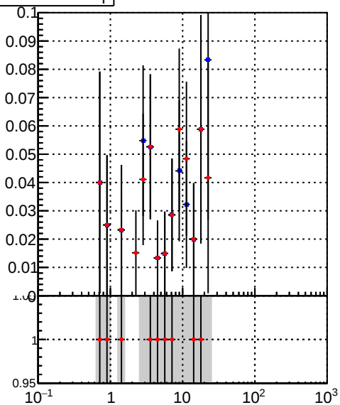
■ DQM_mkFit_time ■ DQM_BDT_mkFit_time
