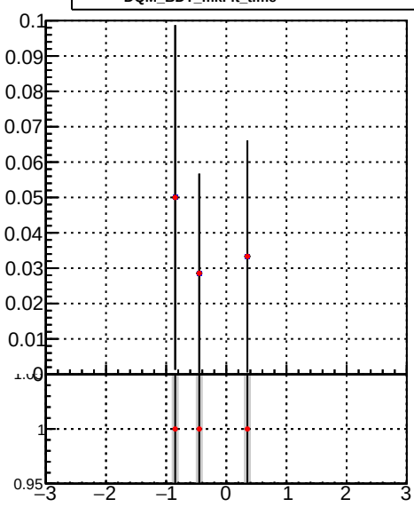
Legend: DQM_mkFit_time (blue square), DQM_BDT_mkFit_time (red circle)
