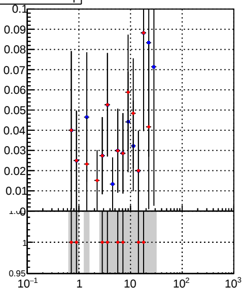
—●— DQM_mkFit_time —●— DQM_BDT_mkFit_time
