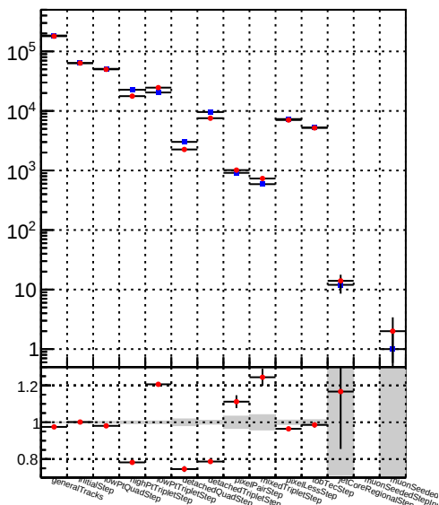
Number of iterations: 1000000 Legend: DQM_mkFit_time DQM_BDT_mkFit_time
