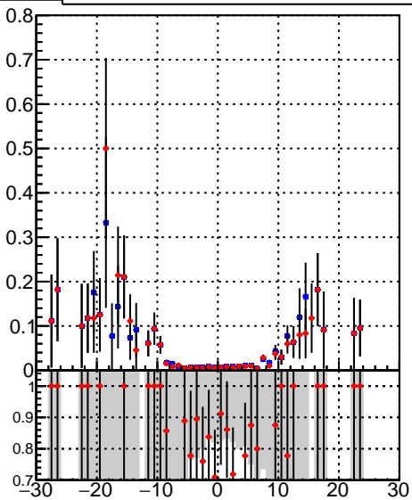
Efficiency vs vert r — DQM_mkFit_time — DQM_BDT_mkFit_time
