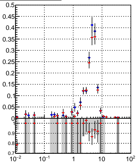
Efficiency vs vert r — DQM_mkFit_time — DQM_BDT_mkFit_time
