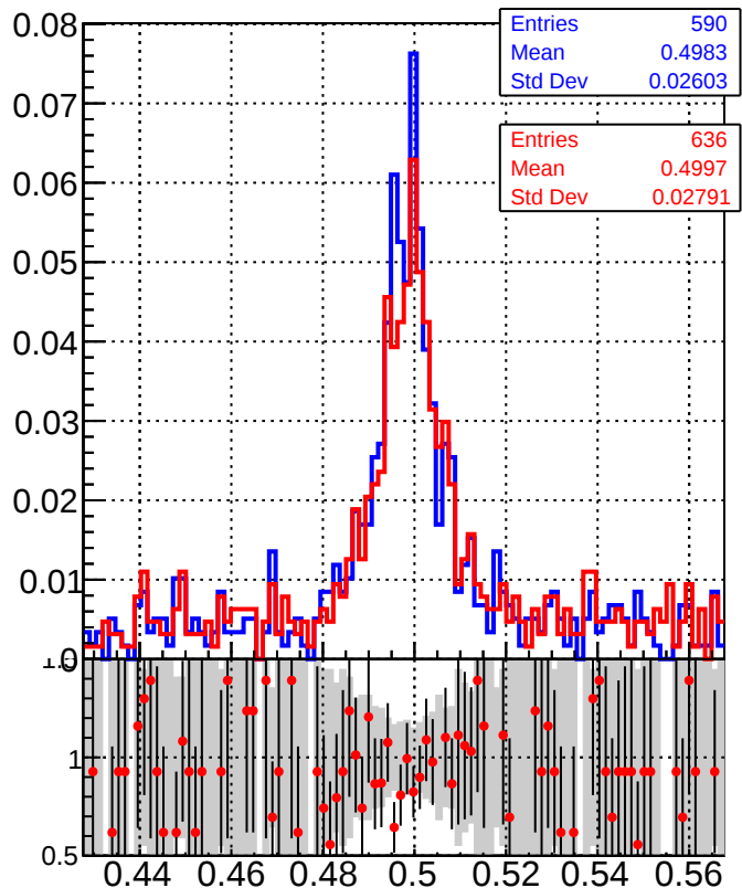
Invariant mass of all K0S
