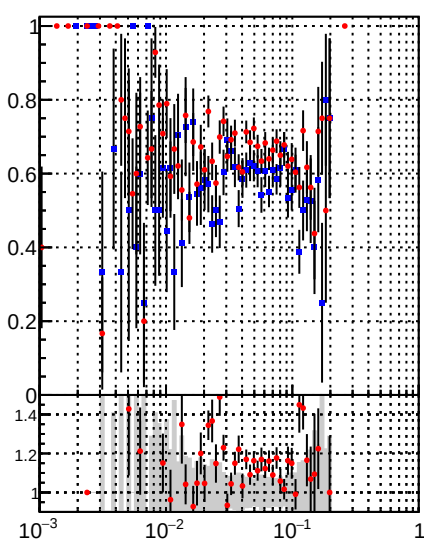
Fake rate vs \sqrt{s} DQM_mkFit_time DQM_BDT_mkFit_time
