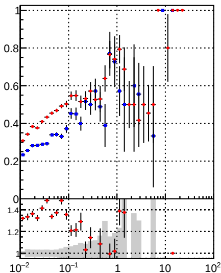
—■— DQM_mkFit_time —●— DQM_BDT_mkFit_time
