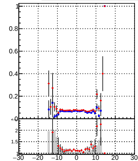
—●— DQM_mkFit_time —●— DQM_BDT_mkFit_time
