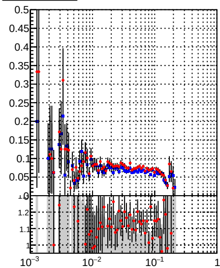
Fake rate vs \epsilon — DQM_mkFit_time — DQM_BDT_mkFit_time
