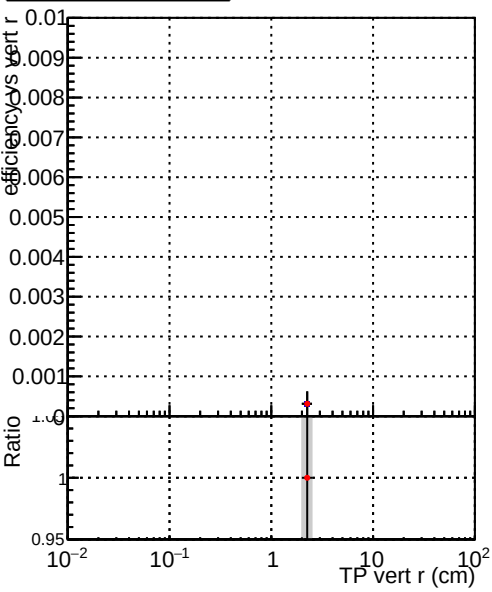
Efficiency vs TP vert r (cm) Legend: DQM_TT_PR43146 DQM_TT_PR43146_swap
