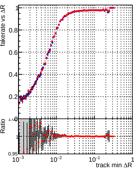
Fake rate vs \Delta R (track, jet) DQM_TT_PR43146 DQM_TT_PR43146_swap
