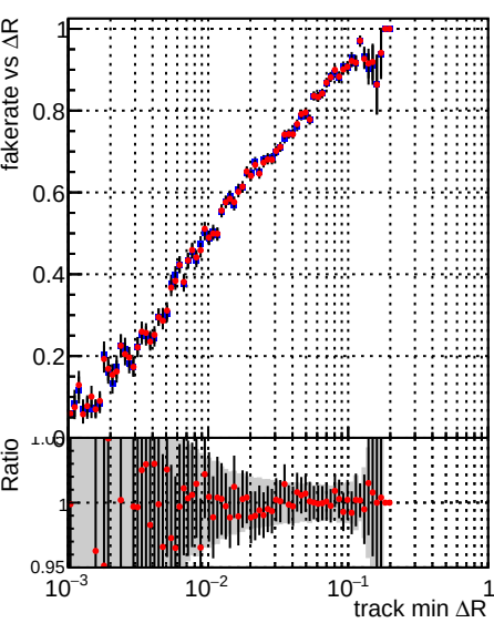
Fake rate vs \Delta R(\text{track, jet}) Legend: \blacksquare DQM_TT_PR43146 \bullet DQM_TT_PR43146_swap
