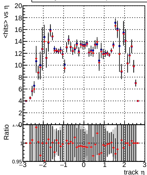
mean hits vs \eta — DQM_TT_PR43146 — DQM_TT_PR43146_swap
