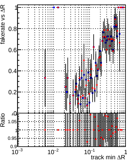
Fake rate vs \Delta R(\text{track, jet}) Legend: DQM_TT_PR43146 (blue squares), DQM_TT_PR43146_swap (red circles)
