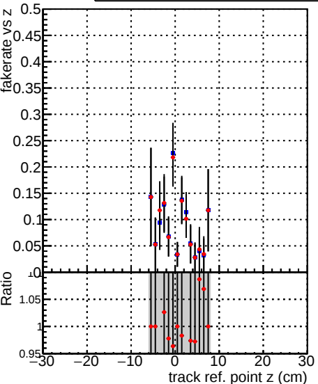
Fake rate vs v DQM_TT_PR43146 DQM_TT_PR43146_swap
